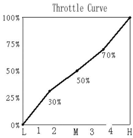
Throttle Curve
