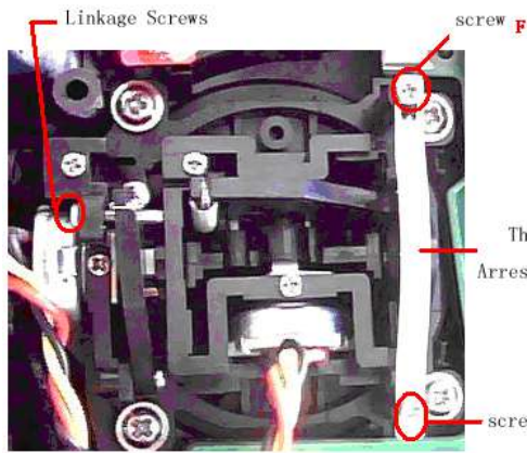
Right Throttle Position
