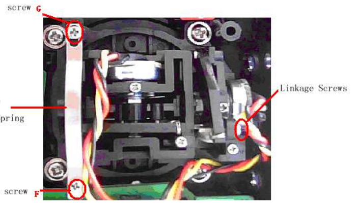
Left Throttle Position
